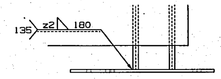
DETAIL AT- K
