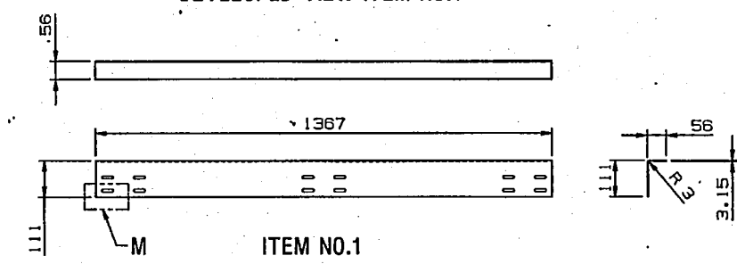
DEVELOPED VIEW ITEM NO.1
