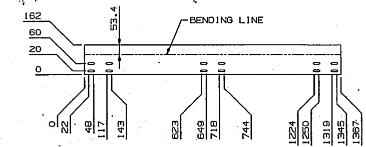
DEVELOPED VIEW ITEM NO.1
