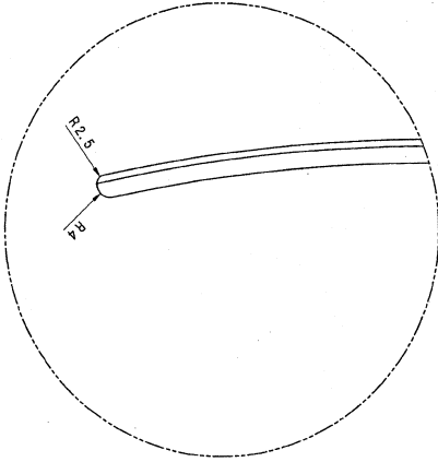
DETAIL AT Z SCALE 1:1
